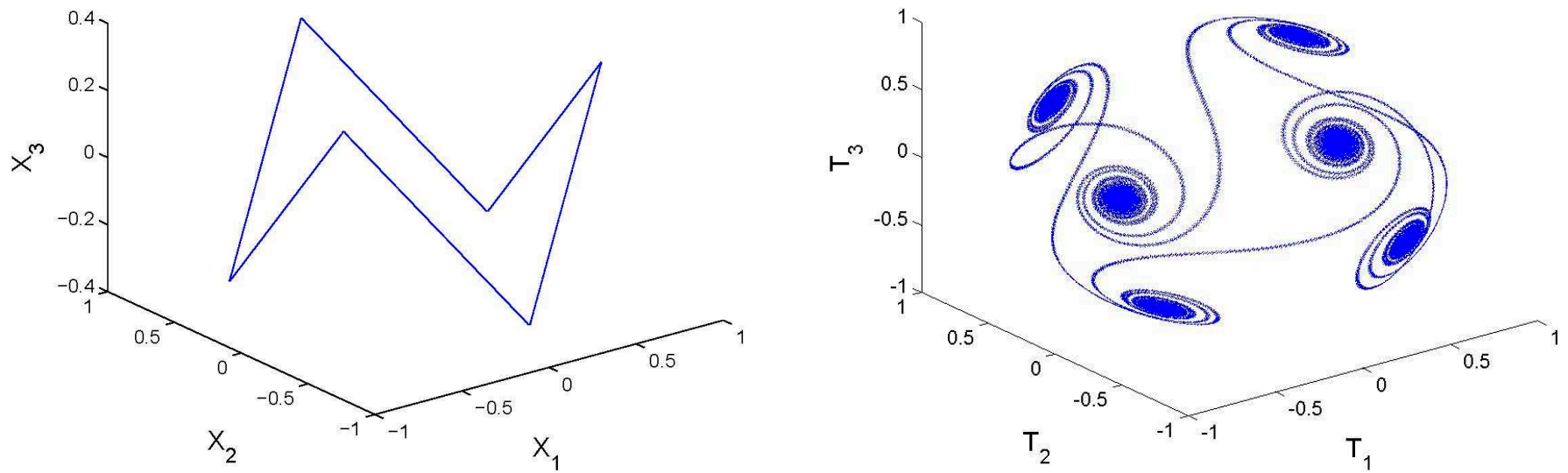
Figure 7: \mathbf{X}_{alg} and \mathbf{T}_{alg} , at t = \frac{2\pi}{9}(\frac{1}{4} + \frac{1}{49999}) .
